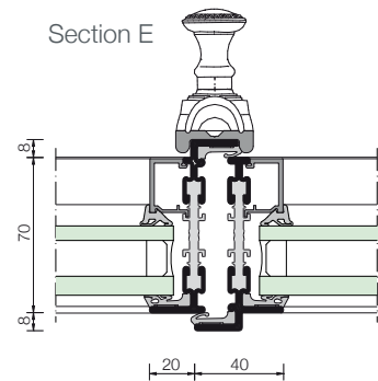
Section E alternative
