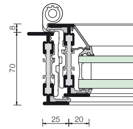
Section A Alternative with slanted glazing bead
