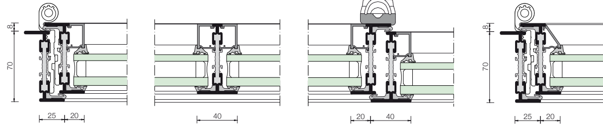
Section A-B Alternative with standard glazing bead
